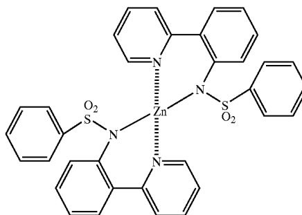
(Compound 2)
