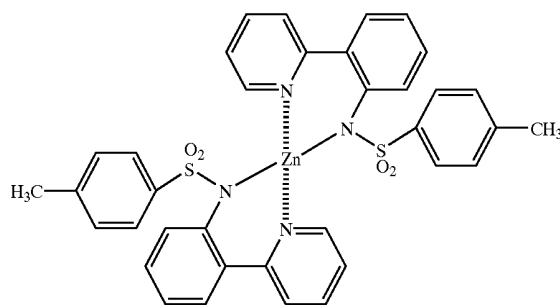
(Compound 3)
